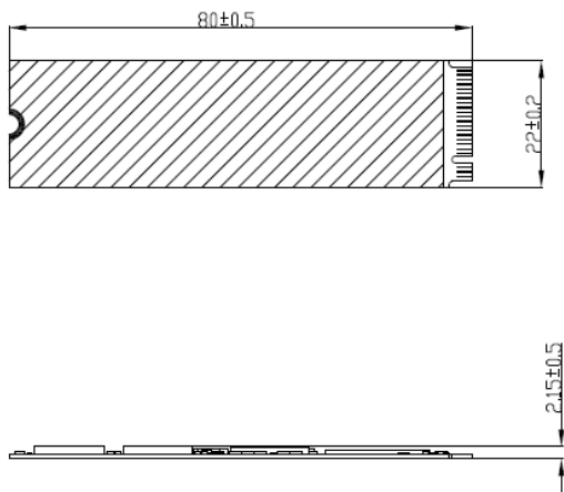
<Without heatsink>
